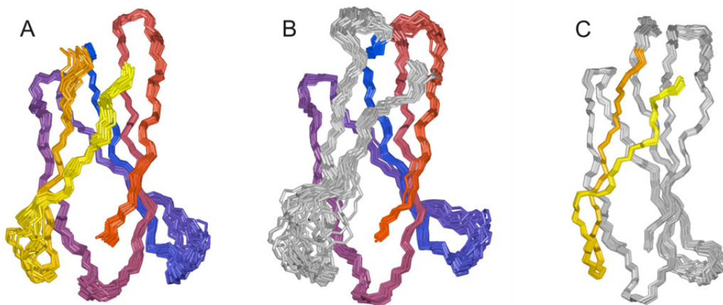
Figure S2. Comparison of the AB:anastellin complex with 1FN3 and 3FN3. (A-C) Superimposed backbone traces of the AB:anastellin complex (residues 813-834 of AB and 638-697 of anastellin) (panel A), 1FN3 (residues 610-697) (panel B), and 3FN3 (residues 813-896) (panel C). The color scheme for the AB:anastellin complex is the same as in Fig. 4, i.e. the color of AB changes smoothly from yellow at the N-terminus to orange at the C-terminus, and the color of anastellin changes from blue at the N-terminus to red at the C-terminus. Residues 638-697 in 1FN3 (panel B) and 813-834 in 3FN3 (panel C) are colored as in panel A to facilitate their comparison with anastellin and AB, respectively. The rest of 1FN3 and 3FN3 is colored gray.
