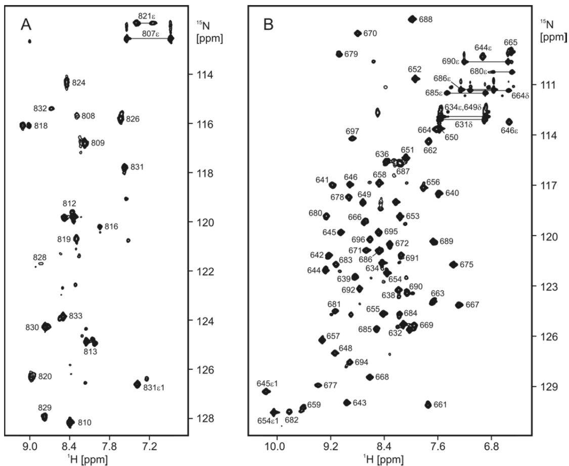
Figure S1. 2D ^1\text{H} - ^{15}\text{N} HSQC spectra of (A) ^{15}\text{N} -labeled AB bound to unlabeled anastellin and (B) of ^{15}\text{N} -labeled anastellin bound to unlabeled AB. The assignments are indicated. Signals from T825 and V828 in AB are very weak, and the former is not observable at this contour level. Signals from G661, R644 \epsilon and R646 \epsilon in anastellin are aliased.
